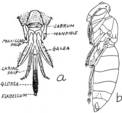
Fig. 102. a, Chewing and lapping mouth parts; b, Pupa of Vespa macutata Kirby.
